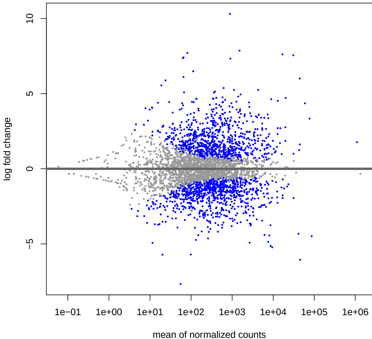
MA-plot for GrowthXMedia: Plate vs Broth
