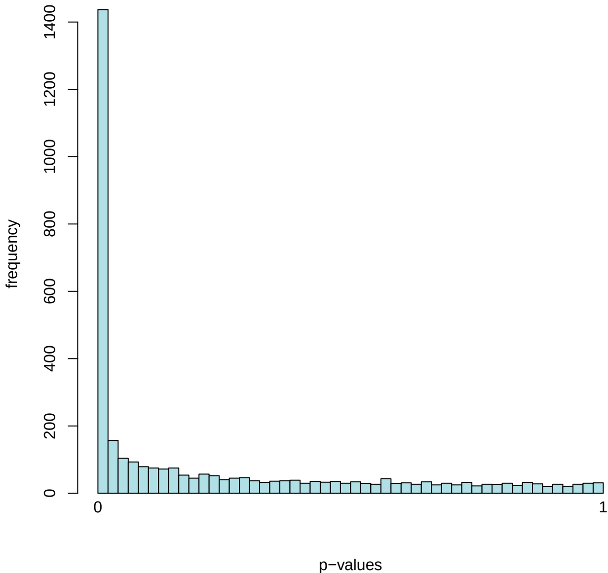
Histogram of p-values for GrowthXMedia: Plate vs Broth
